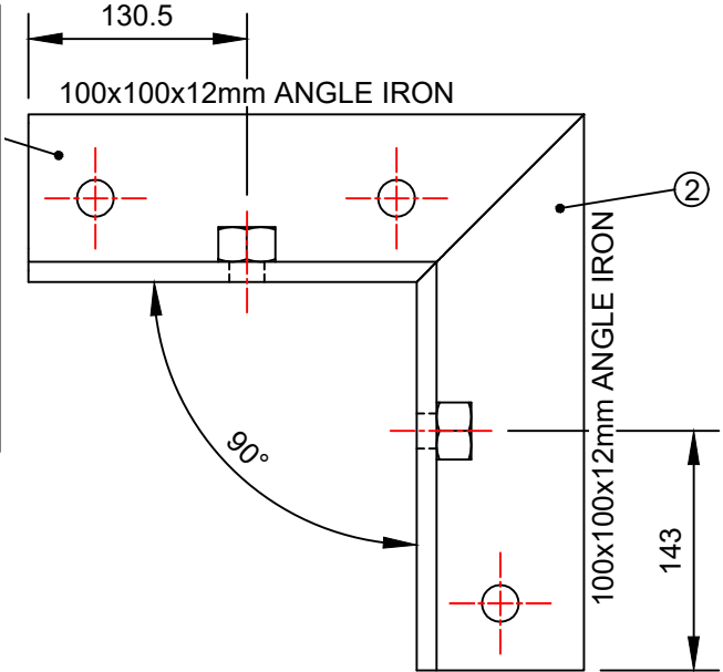
ASSEMBLY PLAN VIEW
