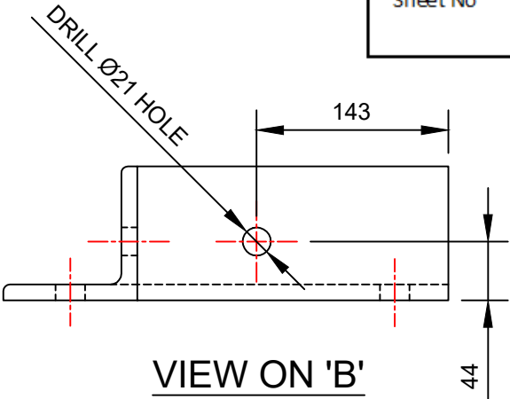
CONTAINER CORNER HOLD DOWN BRACKET - TYPE 'B'
